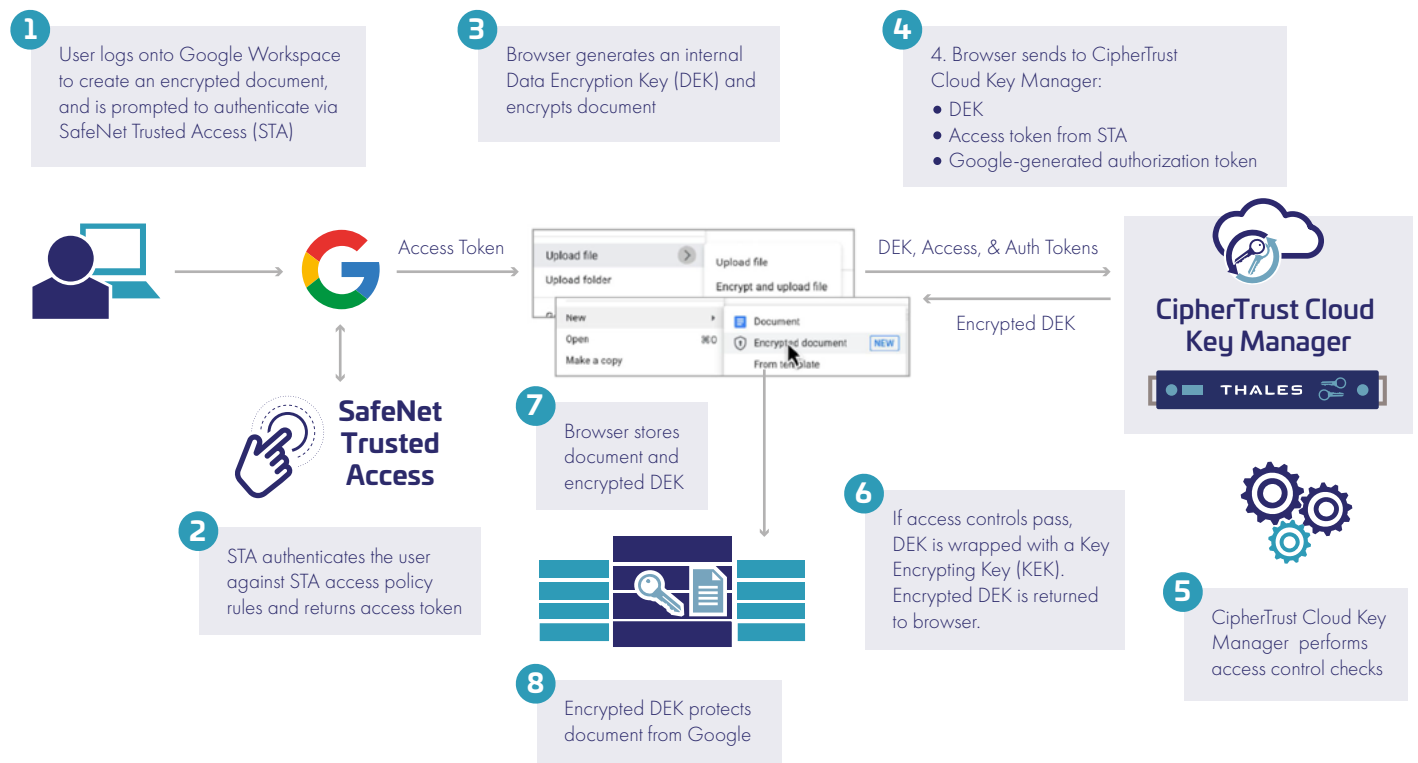
Fig 1. Authentication & Encryption Workflow Pictorially
